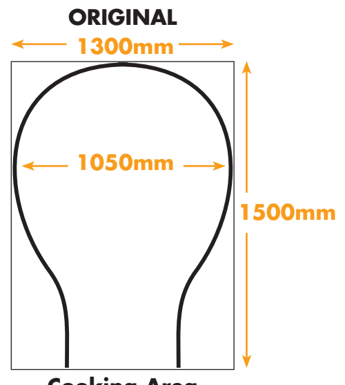
Cooking Area 1050mm wide x 1300mm deep
